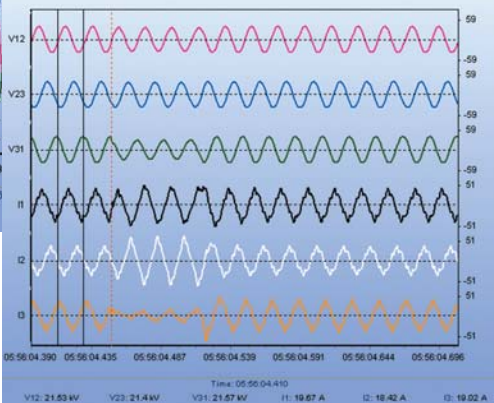
VOLTAGE DIP WITH VECTOR ANALYSIS
