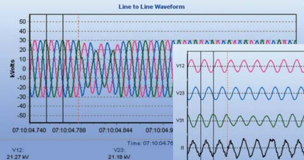
VOLTAGE DIP OVERLAPPED
