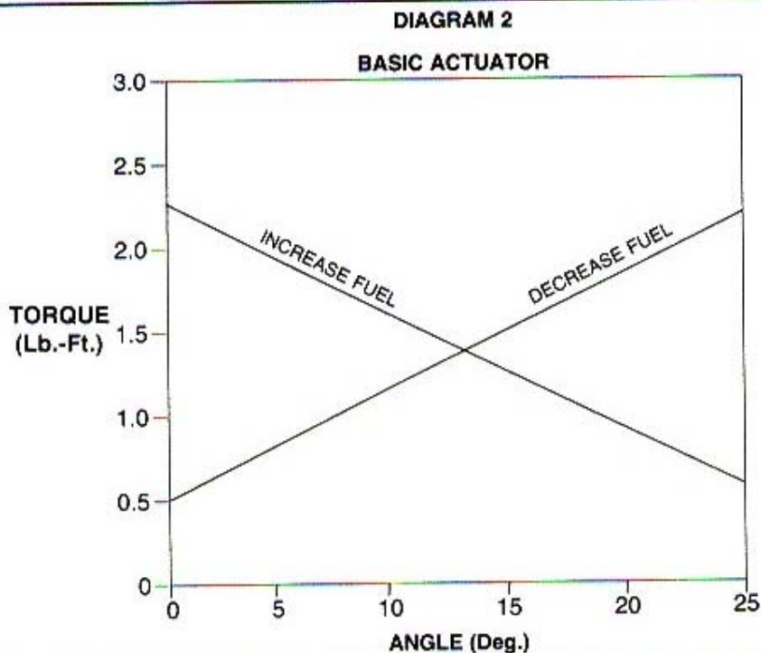
Graph of Actuator Torque
