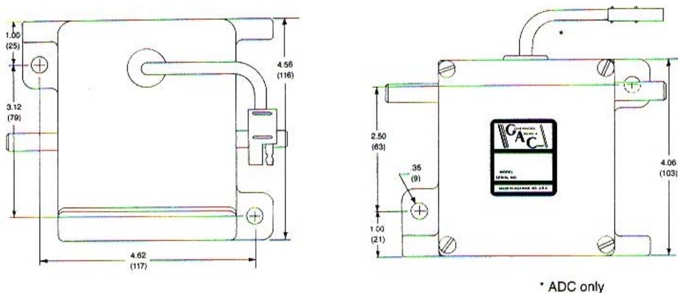
ADB and ADC Actuator Outline Dimensions
