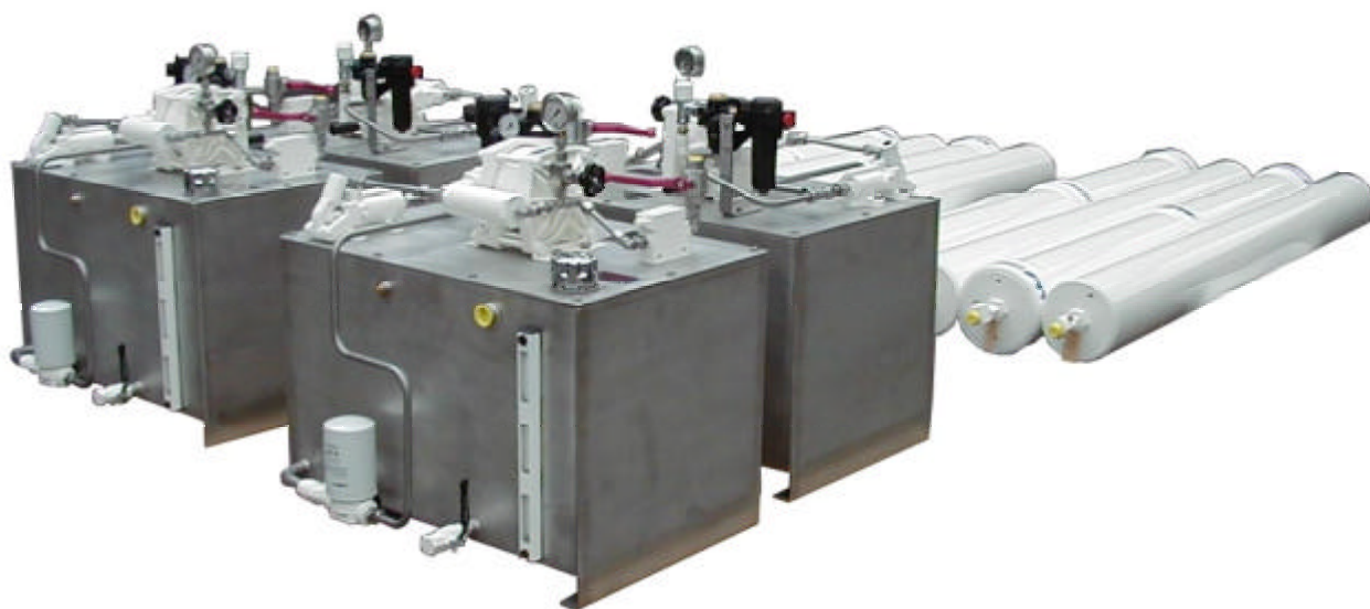
APS starting system, made out of stainless steel. The accumulators are specially painted (see water proof). All components mounted on the tank (Variation A) with the accumulators delivered as loose parts.
