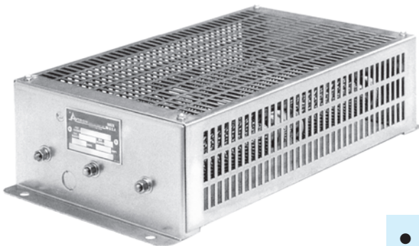
Six Avtron Wirewound Resistors with protective enclosure
