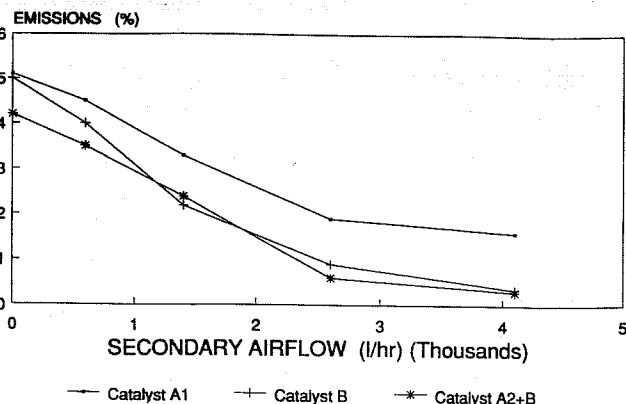
Fig. 23 CO Emissions Versus Secondary Airflow Load = 3kW, Baseline = 4.5%
