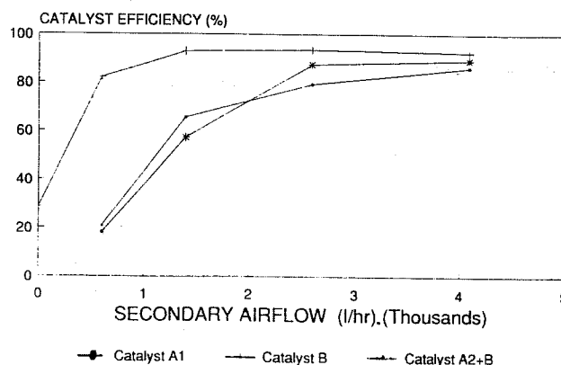
Fig. 19 HC Catalyst Efficiency Versus Airflow Load = 1.5kW
