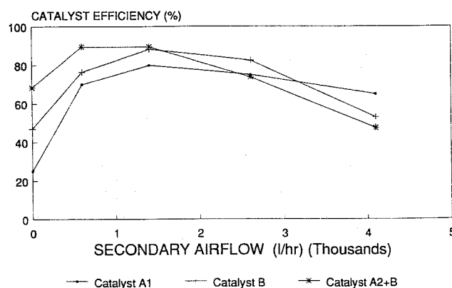
Fig. 14 NOx Catalyst Efficiency Versus Airflow Load = 1.5kW
