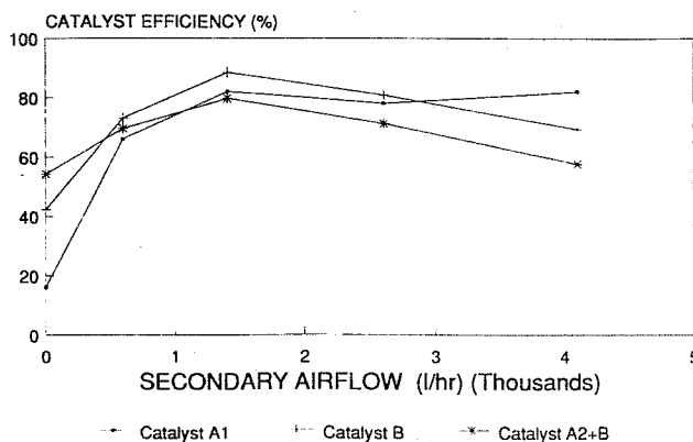
Fig. 15 NOx Catalyst Efficiency Versus Airflow Load = 3kW
