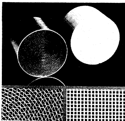
Fig. 7 Metallic Support Versus Ceramic Support
