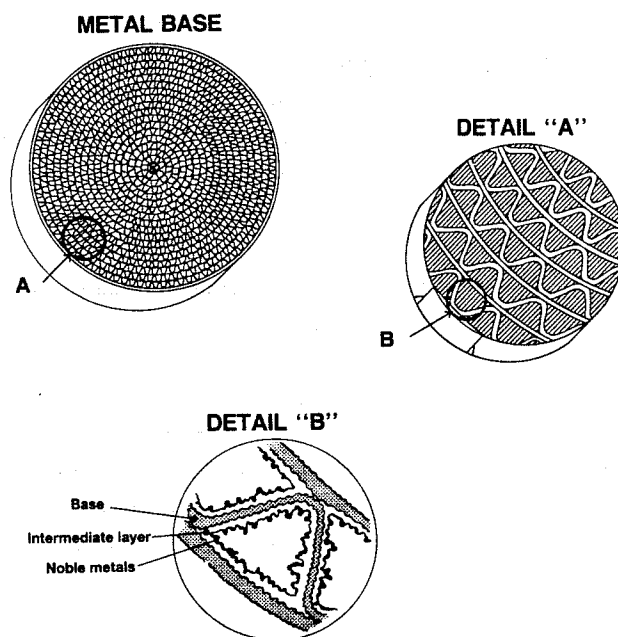
Fig. 4 Catalyst Construction
