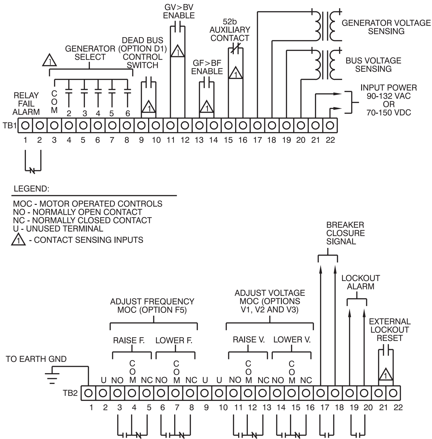
Figure 4 - External Connections
