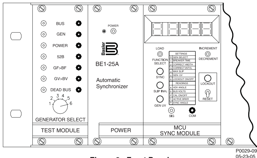
Figure 2 - Front Panel
