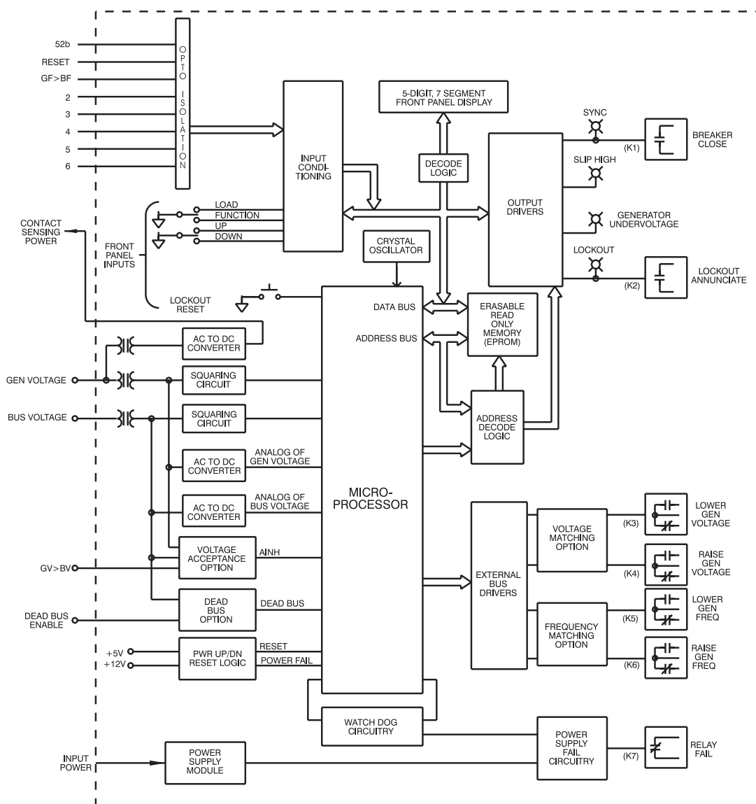
Figure 3 - Function Block Diagram
