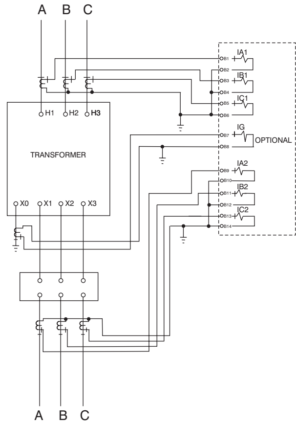
Figure 3 - Typical AC Connections
