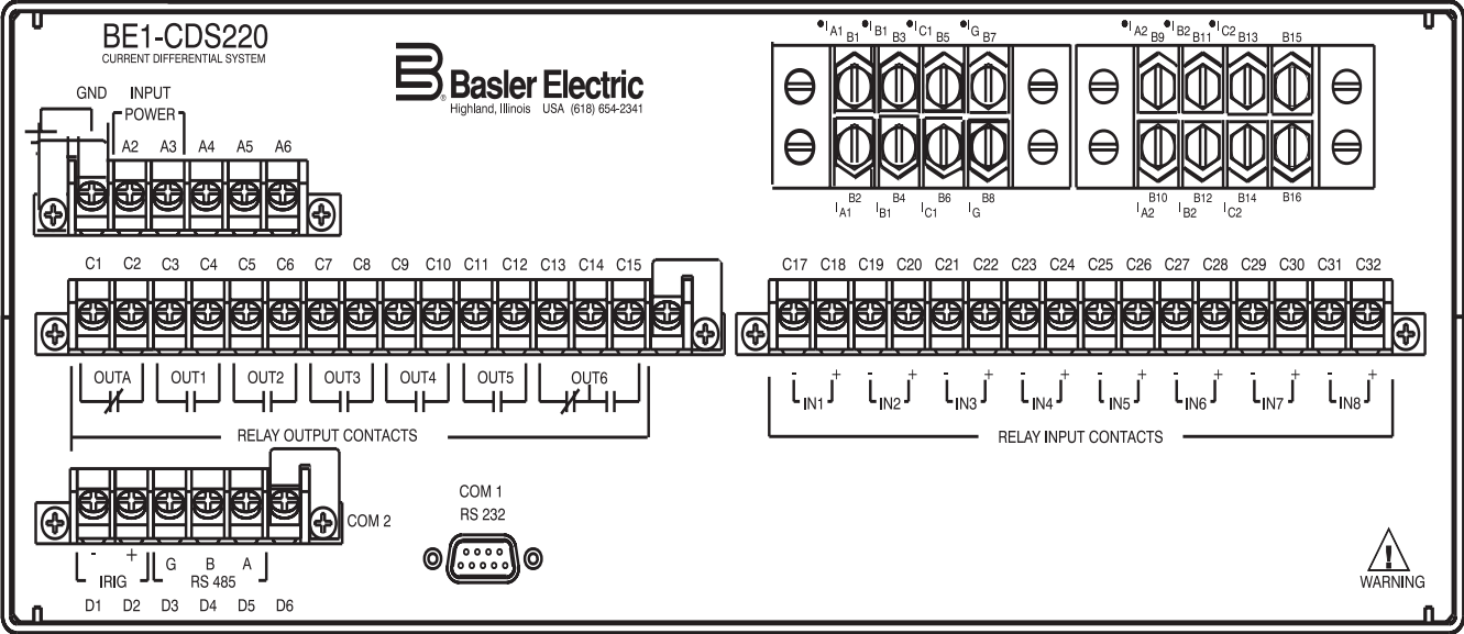
Figure 5 - CDS220 Rear Panel Connections
