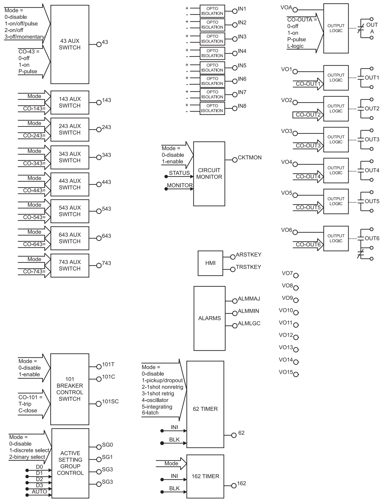
Figure 6A - CDS220 BESTlogic Function Blocks
