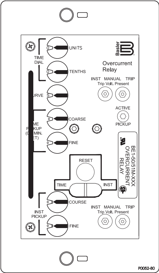
Figure 5 - Front Panel, Vertical Mounting
