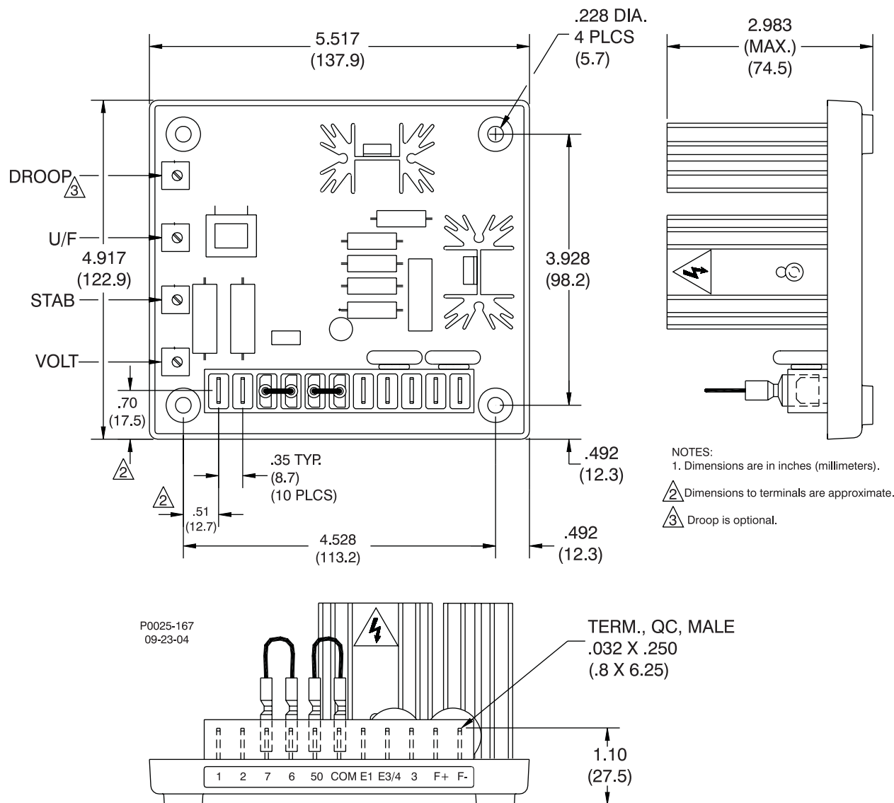
Figure 4 - Outline Drawing
