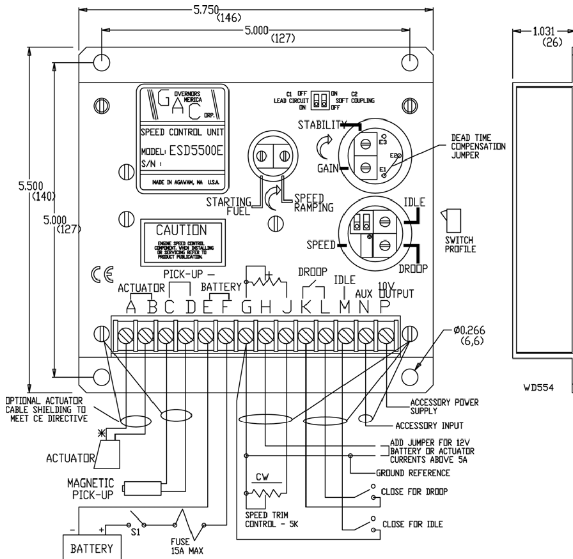
DIAGRAM 1, ESD-5500E Series Wiring Diagram and Outline
