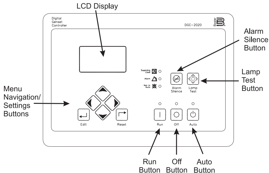
Figure 1 - Front Panel HMI (Human Machine Interface)
