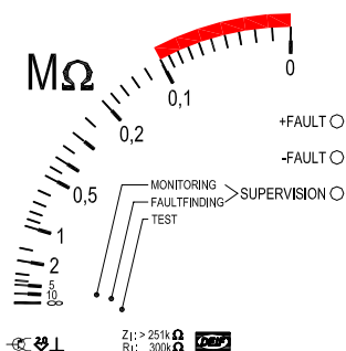
Fig. 2, 10...0MΩ scale
