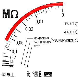
Fig. 1, 1...0MΩ scale
