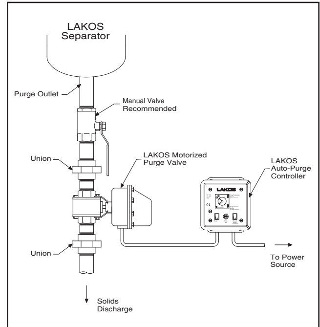
SUGGESTED INSTALLATION
