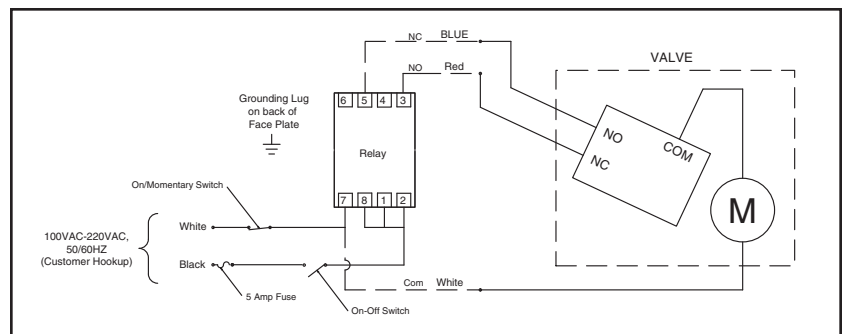
WIRING DIAGRAM
